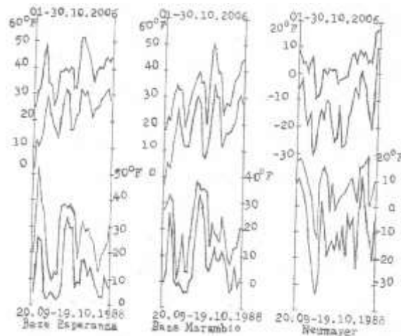
Fig. 6: The Saros meteorological cycle in the evolution of the daily maximum and minimum air temperatures at Esperanza Base, Marambio Base and Neumayer
